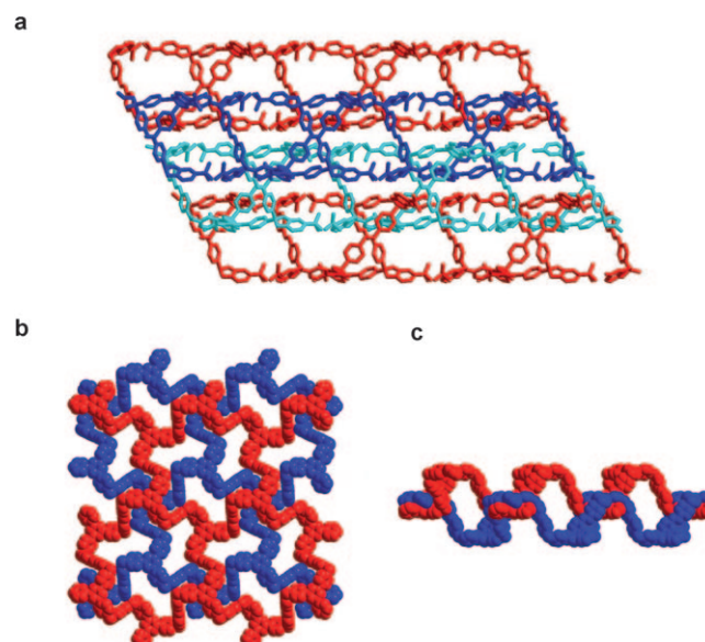
Figure 2. The (A–B–C) n layer structure of 3 in the solid state. a) Wire-frame view along the crystallographic x axis. b, c) Space-filling representation of two adjacent layers viewed along the crystallographic z and y axes. The layers are tightly interwoven, but there is no catenation. For clarity, the catechol groups have been removed in (b) and (c).
